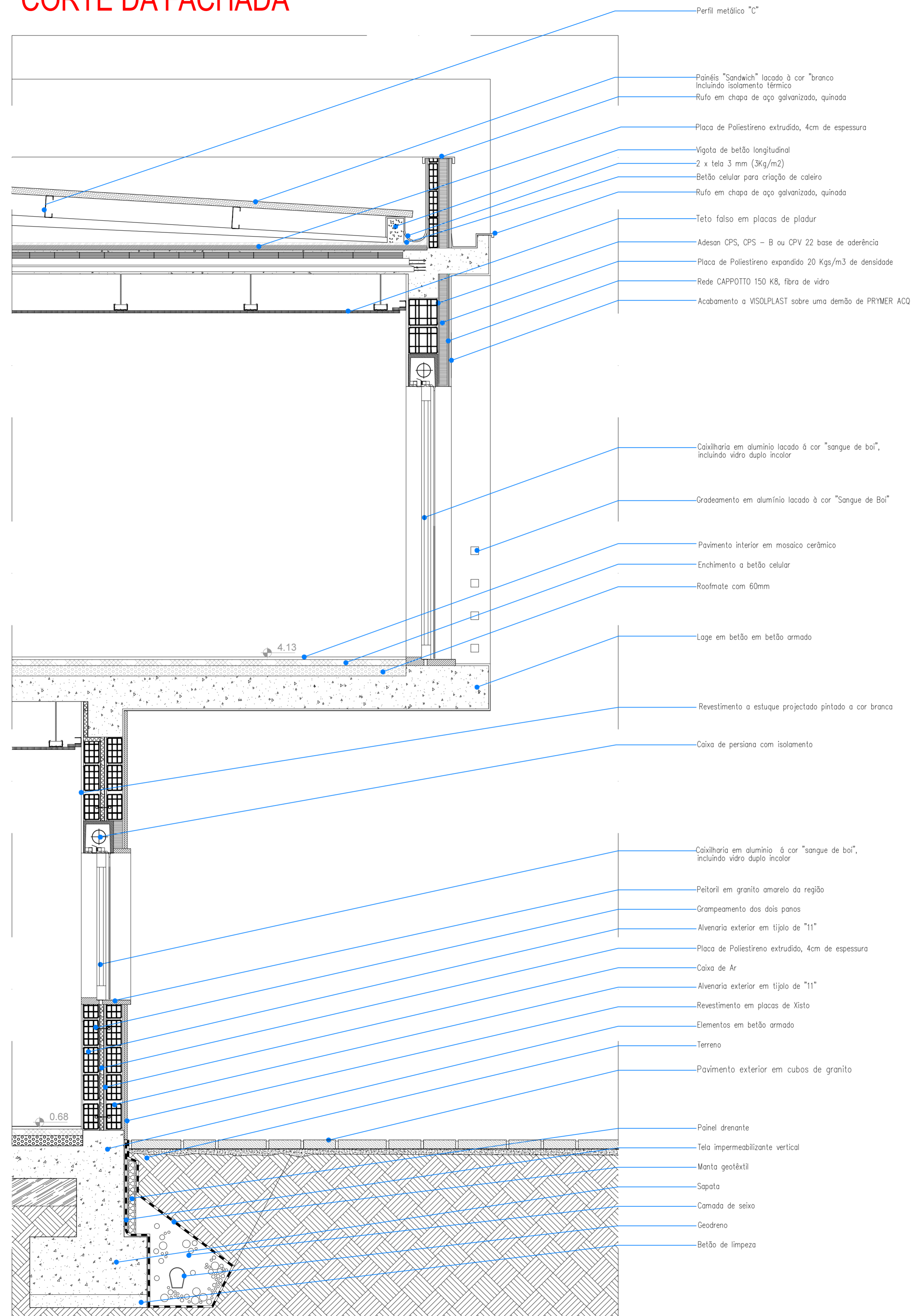
PORMENOR 2 Esc: 1/20
