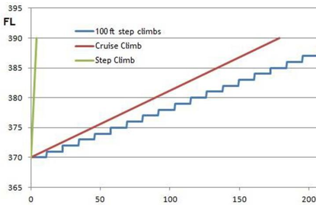
Figure 2: Time needed for a 2.000ft altitude change for an A330
