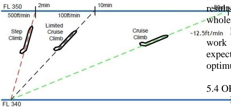
Figure 3: Time needed for a 1.000ft altitude change for a B757
