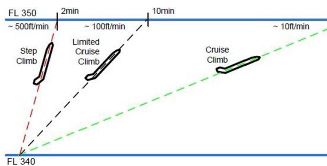
Figure 1: Difference between cruise climb, limited cruise climb, and regular step climb (SESAR, 2010a)
