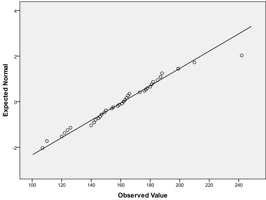
Normal Q-Q Plot of TCTotal
