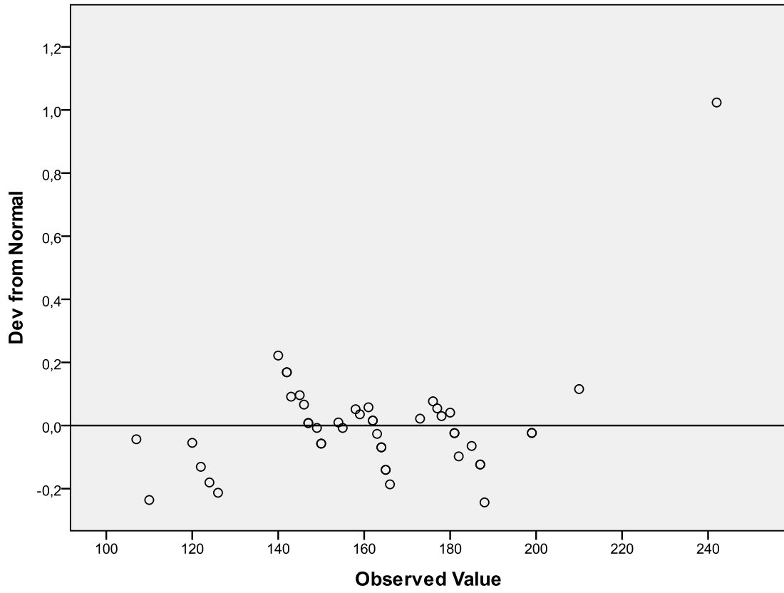
Detrended Normal Q-Q Plot of TCTotal
