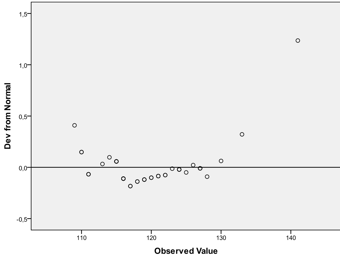
Detrended Normal Q-Q Plot of ACTotal
