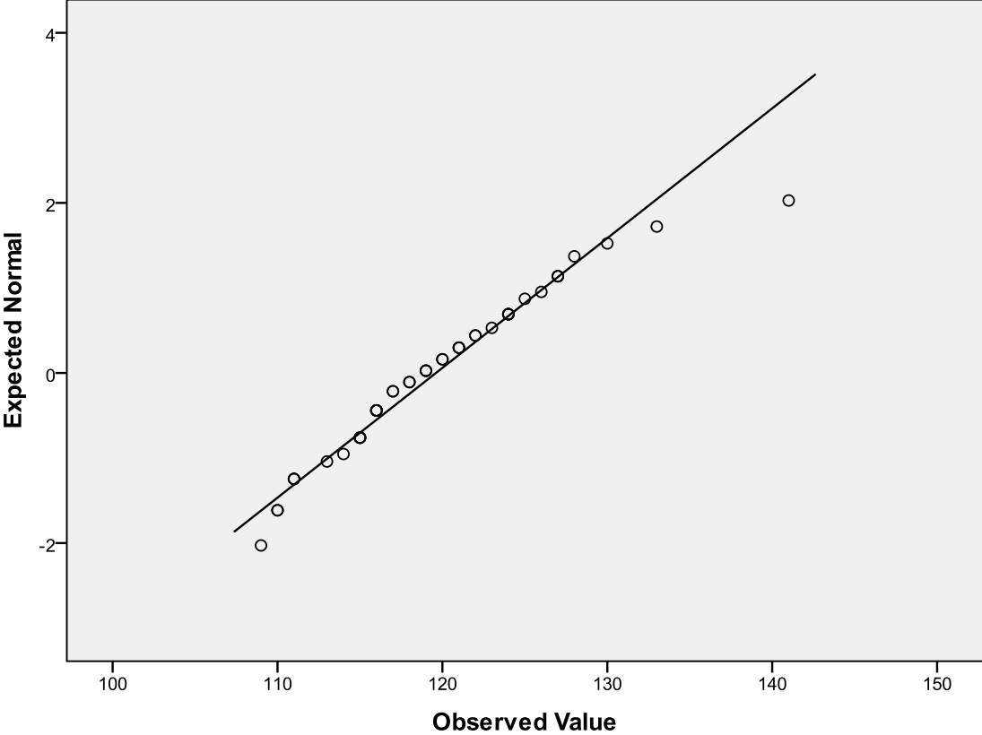
Normal Q-Q Plot of ACTotal
