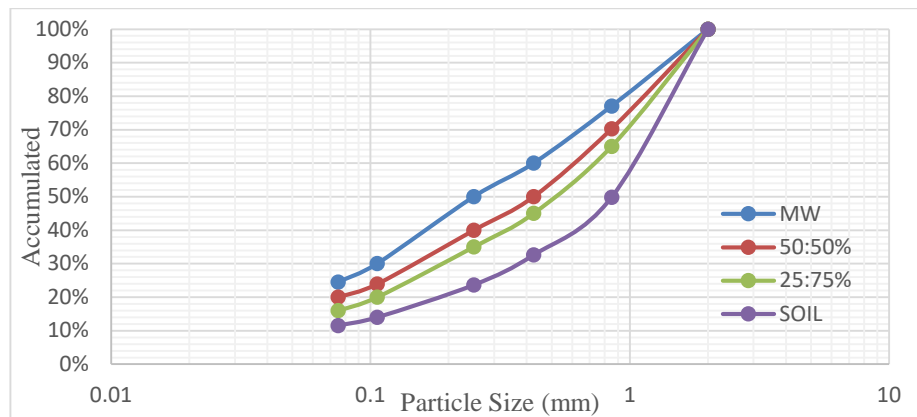
Fig. 1: Granulometry distribution.
