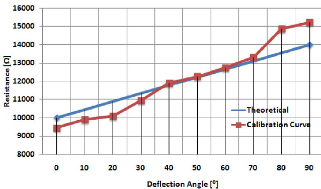
Fig. 5. Theoretical and Calibration curve of Flex sensor.
