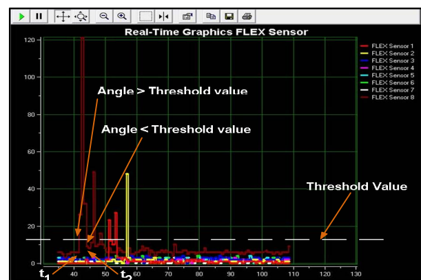
Fig. 10. Real-time graphics Flex Sensor plot.
