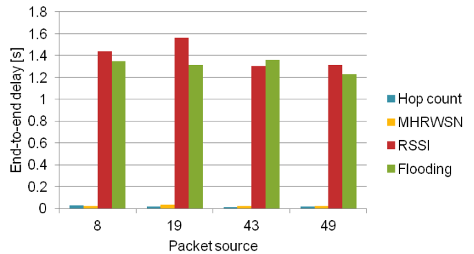
Fig. 4. Total average end-to-end delay experienced by the packets.
