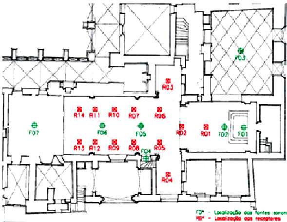
Fig. 11. Scheme of the positioning of the sound sources (in green) and receivers (in red).
