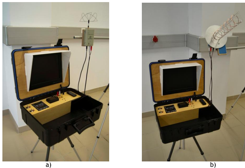
Figure 1- Complete ground control station showing the video receiver connected to: a) skew planar wheel antenna and b) heliaxial high directivity antenna.
