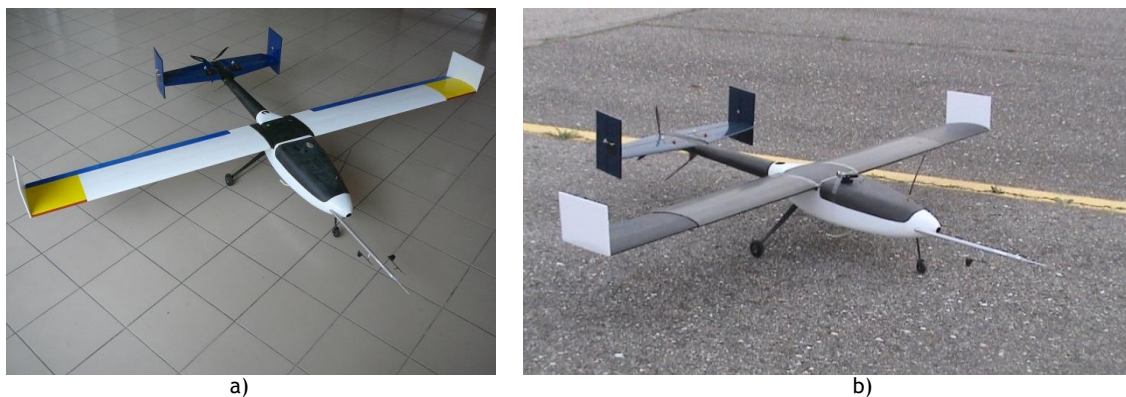
Figure 7-Olharapo UAV fitted with: a) Conventional fixed wing and b) Variable-span wing
