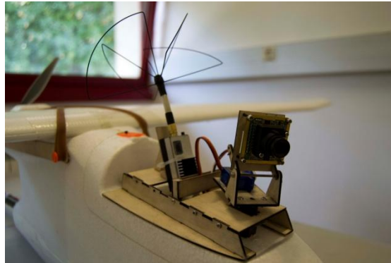
Figure 2-Detachable pod carrying the airborne FPV system components
