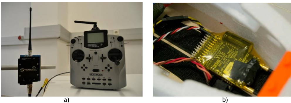
Figure 3- Complete long range radio control system showing: a) the radio controller and the LRS transmitter, and b) LRS receiver.
