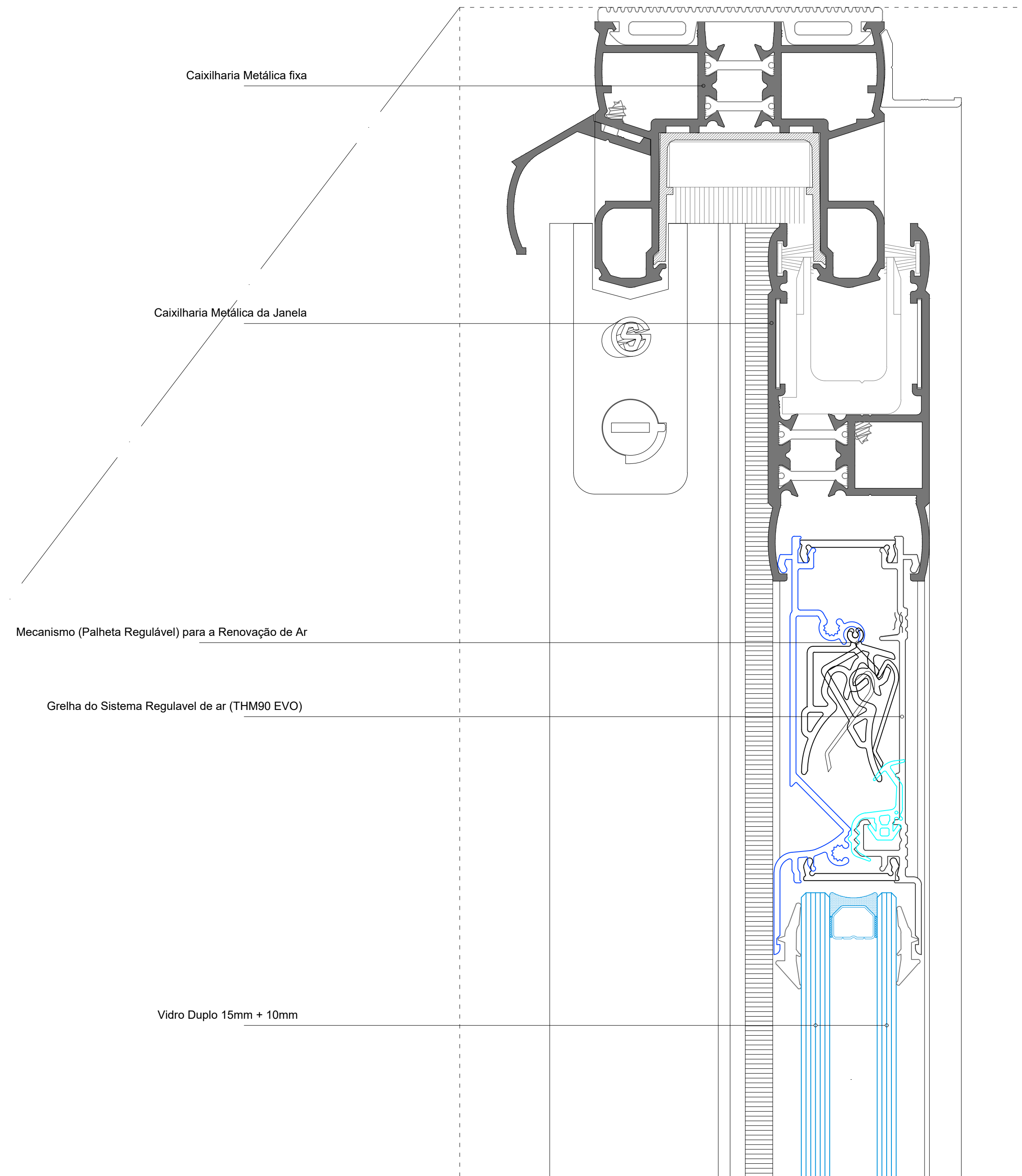
Pormenor 5
