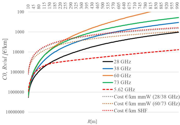
Fig. 6. Network revenue/cost per unit length per year as a function of R , with R_{max} = 1000 m.
