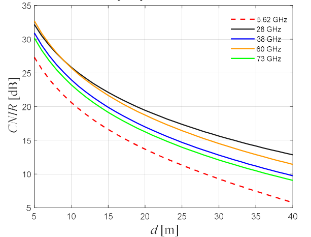
Fig. 2. Variation of the CNIR with the distance d for the 5.62, 28, 38, 60 and 73 GHz frequency bands for R = 400 m.
