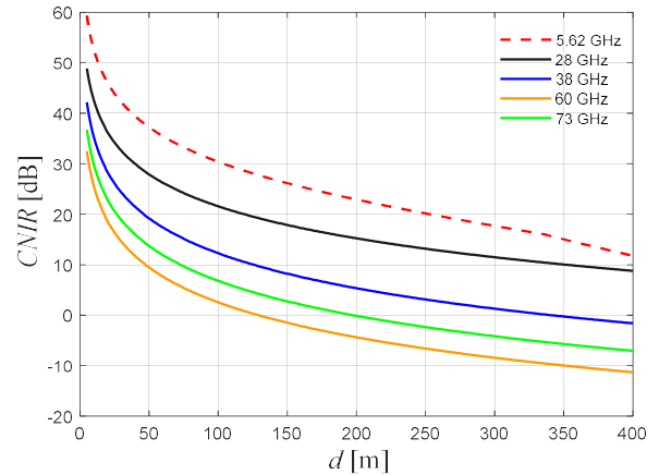
Fig. 2. Variation of the CNIR with the distance d for the 5.62, 28, 38, 60 and 73 GHz frequency bands for R = 400 m.
