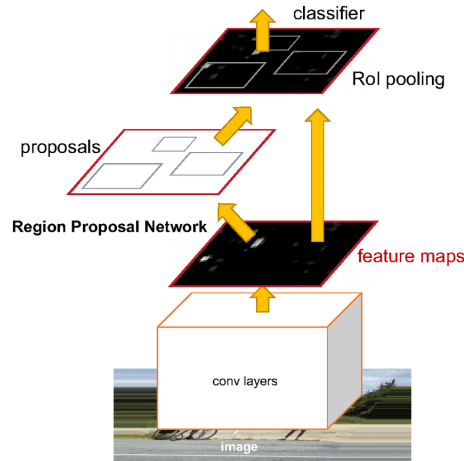
Figure 2.6: Faster R-CNN pipeline [GS15]. The two main modules are the RPN, to predict where an object might be, and the R-CNN detector, to classify the proposed regions.
