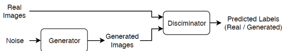
Figure 2.9: Typical GAN architecture [Mat20]. The generator takes random noise as input and outputs fake, but realistic images. By the end of training, the fake images should be hard to distinguish from the real ones.
