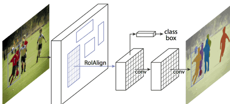
Figure 2.8: Mask R-CNN architecture [DG17]. Built on top of Faster R-CNN, this architecture favours segmentation and includes alignment techniques to ensure optimal mask quality.
