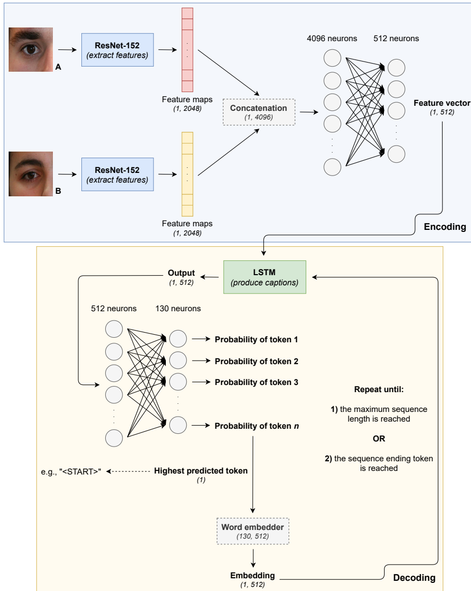
Figure 3.6: In inference mode, the encoding stage is kept: two feature maps are derived, concatenated and compressed further into a 512-dimensional feature vector. Unlike before, the decoding starts with the LSTM receiving the feature vector as is and, in conjunction with two linear layers, outputting the most probable token to start a sentence (ideally, "<START>"). The predicted token is fed to the embedder and the resulting representation is fed back to the LSTM, completing a loop. To exit said loop, one of two conditions must be met: either the maximum sequence length is reached or the "<END>" token is output.
