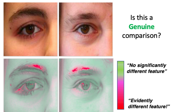
Figure 1. Key insight of the proposed visual explainable framework: given a pair of images, the system not only reports a binary decision ("genuine"/"impostor" classes), but also highlights the regions in each sample that contributed the most in case of a non-match decision . In this example, yet the iris and skin colour are similar between samples, the eyebrows and eyelashes shapes are evidently different, along with a skin spot in the sample illustrated at the left side. These are exactly the regions highlighted in the visual explanations.
