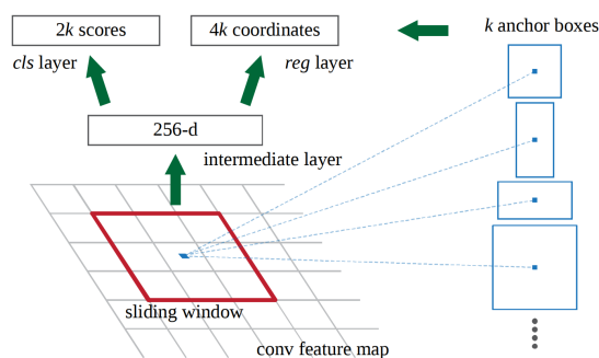
Figure 2.7: Visualisation of the proposed RPN [GS15]. By using multiple anchors with different aspect ratios and sliding them over the received feature maps, the network is able to extract several fixed-length vectors, which are later used for classification and regression.
