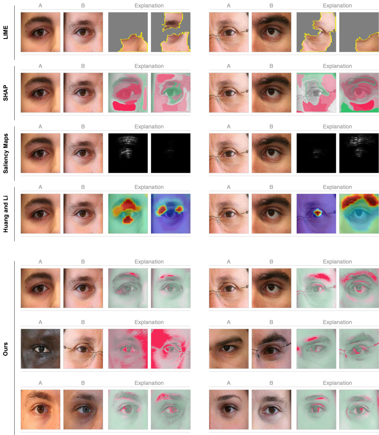
Figure 3. Examples of the results attained by three standard interpretability techniques (LIME, SHAP and Saliency Maps), a state-of-the-art interpretable deep model for fine-grained visual recognition (i.e., [5]) and our method. Notice how our results are clearer in highlighting the components that justify every non-match decision (e.g., skin texture and color, eyebrows/eyelashes size and distribution, irises color and even skin spots).
