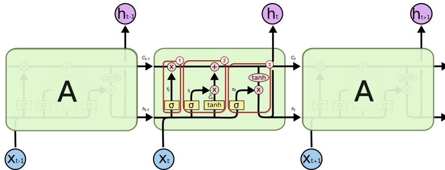
Figure 2.14: Representation of an LSTM's inner workings (edited for explaining purposes) [Ola15]. The top pathway represents the accumulated context (or cell state), which will be subjected to changes if it proves beneficial. In the lower portion of the schematics, two main steps are responsible for filtering and updating the cell state, based on the new information that the unit receives. Finally, the output is a combination of both the updated context and the new, short-term information.
