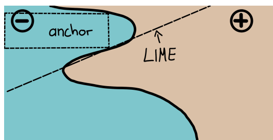
Figure 2.22: A comparison between LIME and anchors [SG18]. One can see that, while LIME tries its best to approximate the decision boundary's behaviour, an anchor provides a more realistic result.
