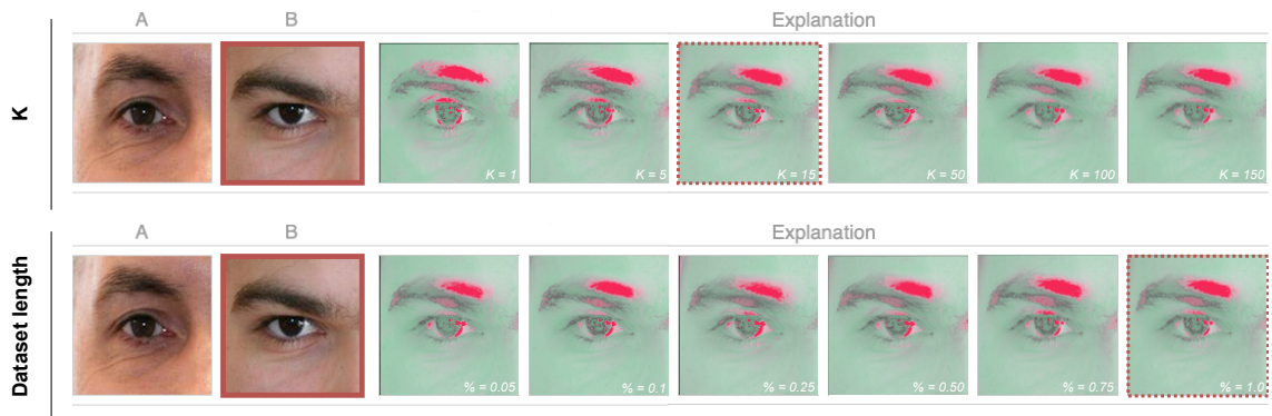
Figure 4.9: Typical changes in the results when the two most important parameters of the proposed method are varied. The red square indicates which image is being explained (i.e., B ), while the red dashed squares provide the default values used in our experiments. In general, increasing K up to 15 allows for smoother explanations, as does keeping a large dataset. Reducing the latter tends to produce less sensitive results, substantially decreasing the plausibility of the visual explanations.
