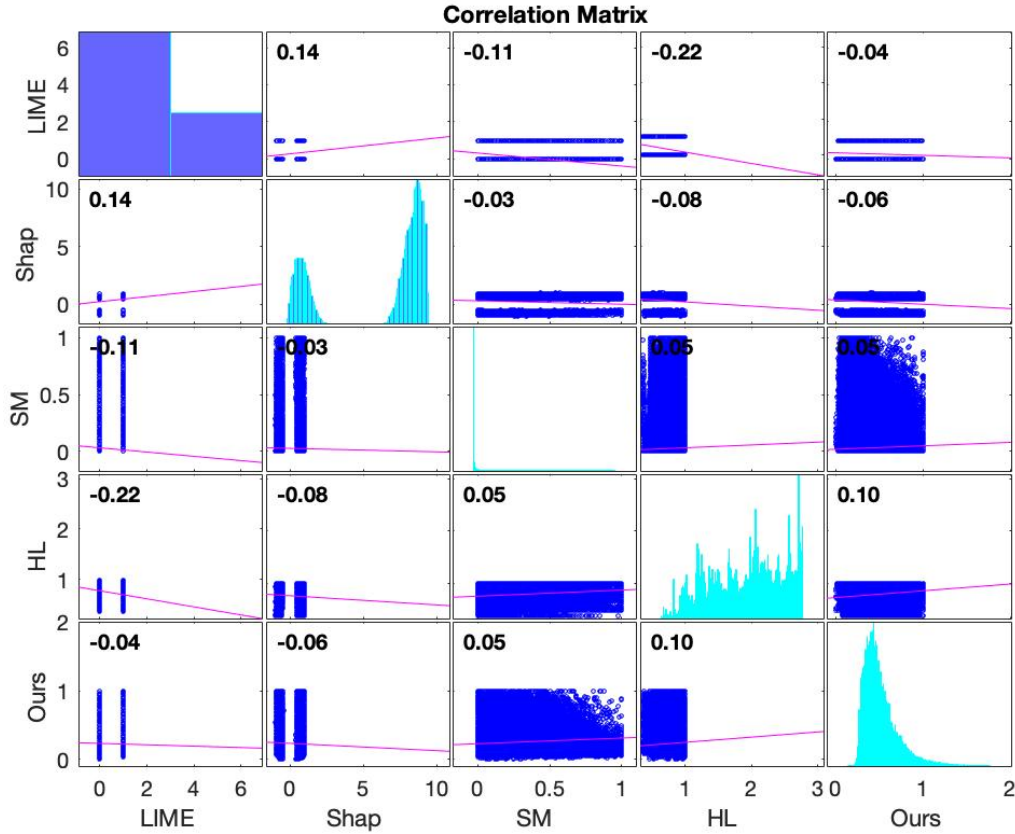
Figure 4.7: Pearson correlation values between the pixel-wise responses provided by the method proposed in this document (Ours) and four baselines techniques (LIME, SHAP, Huang and Li (HL) and Saliency Maps (SM)).
