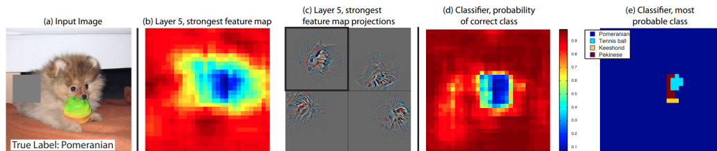
Figure 2.19: Another example of Occlusion Maps being used to interpret a model's decisions [ZF14]. The rightmost figure shows how the predicted class varies with respect to occlusions.
