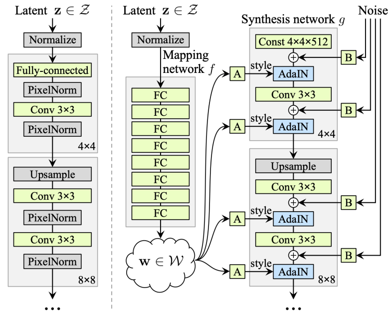
Figure 2.10: StyleGAN architecture [LA19]. On the left, we have the ProGAN architecture, while on the right we have the proposed StyleGAN version with the mapping network and style injection.
