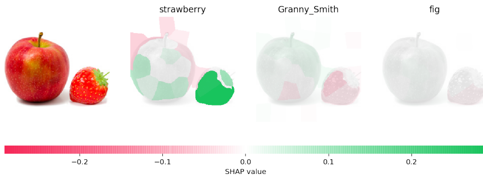
Figure 2.24: KernelSHAP's explanations of a CNN's predictions when given an image from the ImageNet dataset [LL17]. Green super-pixels have higher Shapley values and thus contribute more to the predicted class (unlike super-pixels marked with red tones - this behaviour is inverted in subsection 4.2.1).
