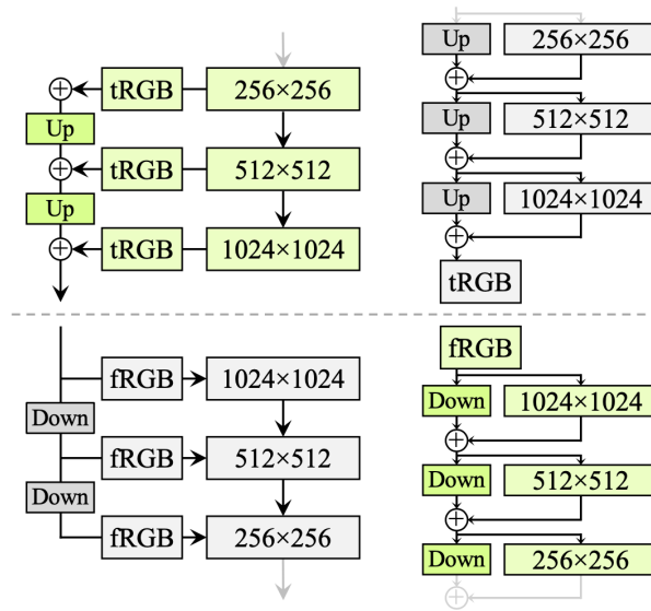
Figure 2.12: Proposed revisions of the networks' architectures [LA20]. On the left, we have input/output skip connections and, on the right, residual style connections. After some experiments, the authors settled on a skip generator (top-left) combined with a residual discriminator (bottom-right).
