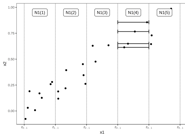
Figure 2.16: Calculation of ALE for feature x_1 , strongly correlated with feature x_2 [Mol19]. The distribution is divided into intervals and, for each one, we determine the difference in predictions when feature x_1 takes on the values of the lower and upper limits. These results are later accumulated (i.e., summed) and centred.
