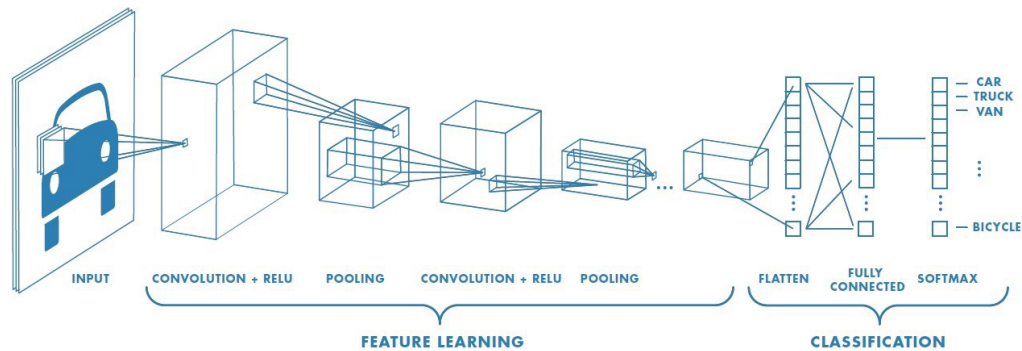
Figure 2.1: Typical CNN architecture [Pra18]. The feature extraction stage extracts as many characteristics as possible from the input image, while the classification stage gives them meaning (i.e., a class).
