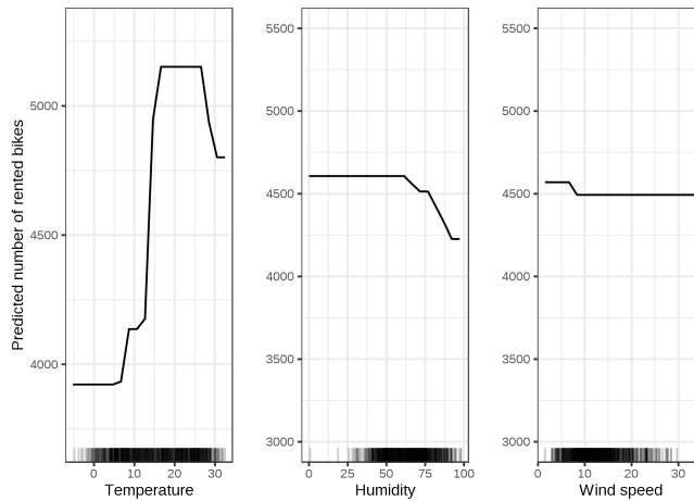
Figure 2.15: Three PDPs from a regression model with three independent variables and one, dependent variable [Mol19]. The predicted values come from a marginalised model ( \hat{f} ) that only relies on one feature.
