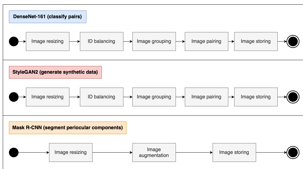
Figure 3.1: Diagram of the data pre-processing pipeline. The images are resized, processed and stored in proper folders.
