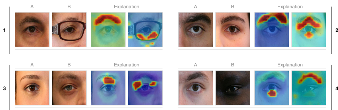
Figure 4.5: Impostor pairs explained with the method by Huang and Li. Such method produces heat maps in which red areas are the most significant.
