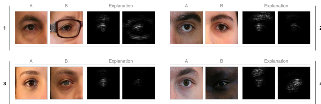
Figure 4.2: Impostor pairs explained using Saliency Maps. Whiter tones highlight areas that justify the predicted class.
