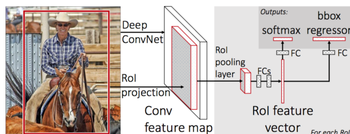
Figure 2.5: Fast R-CNN pipeline [Gir15]. The revision of R-CNN uses a common feature map, shared by all region proposals, instead of extracting features for each and every proposal.
