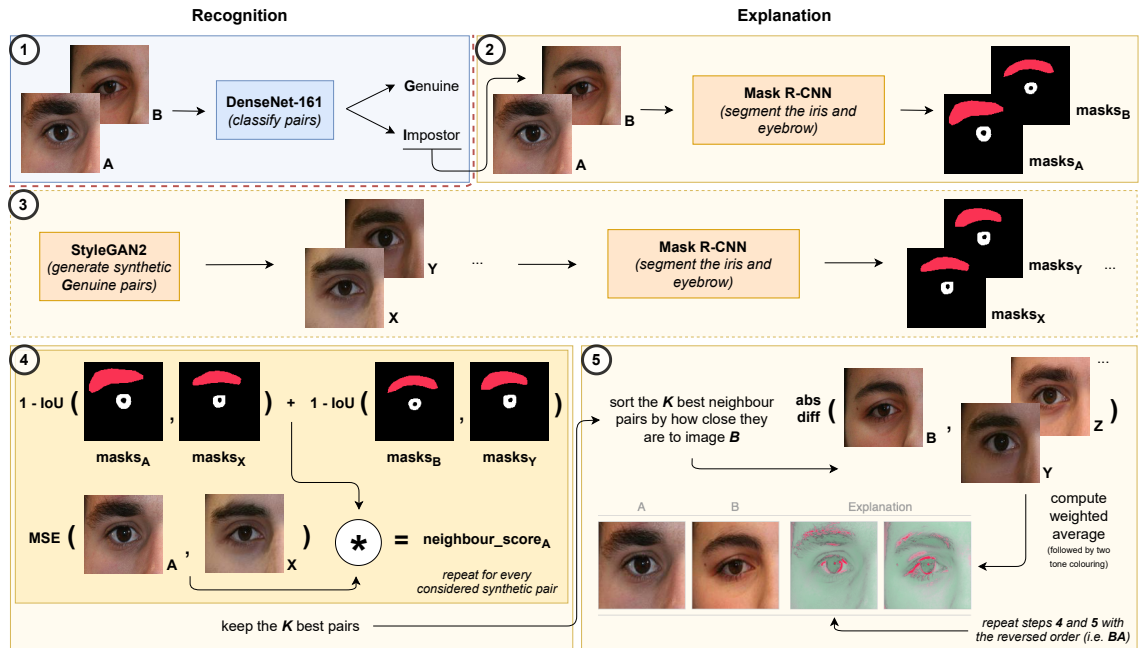
Figure 3.2: Cohesive perspective of the main pipeline of the proposed solution. The recognition step encompasses a CNN that distinguishes between "genuine" and "impostor" pairs. Then, upon an "impostor" decision, steps two to five (explanation) find the K "genuine" synthetic pairs amongst a large set that most closely resemble the query pair. Assuming the alignment between the query and the retrieved pairs, the element-wise differences between the query and a weighted average of the retrieved elements provides a visual explanation of the features in the query that would have to be different to turn it into a "genuine" pair.
