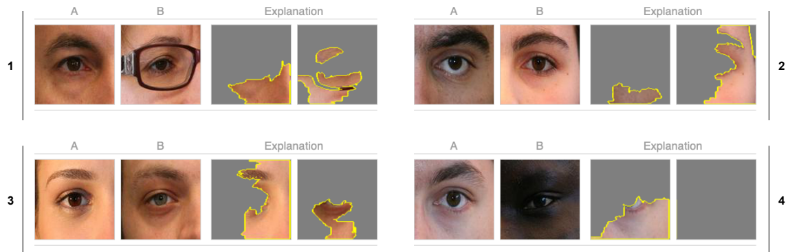
Figure 4.3: Impostor pairs explained with LIME. As mentioned earlier, LIME keeps the most favourable super-pixels and replaces the remaining ones with a solid colour.
