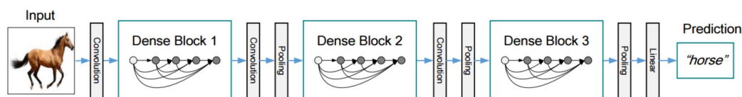
Figure 2.2: Deep DenseNet with three dense blocks [MW17]. Each one of those blocks contains a series of convolutions, pooling and/or BN layers.
