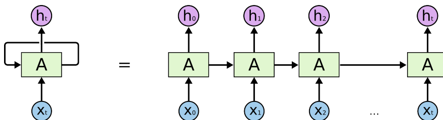
Figure 2.13: Visualisation of a single unit from a RNN [Ola15]. On the left, the unit is seen as theory describes it, while on the right, the loop is expanded indefinitely to form a chain (for explaining purposes).
