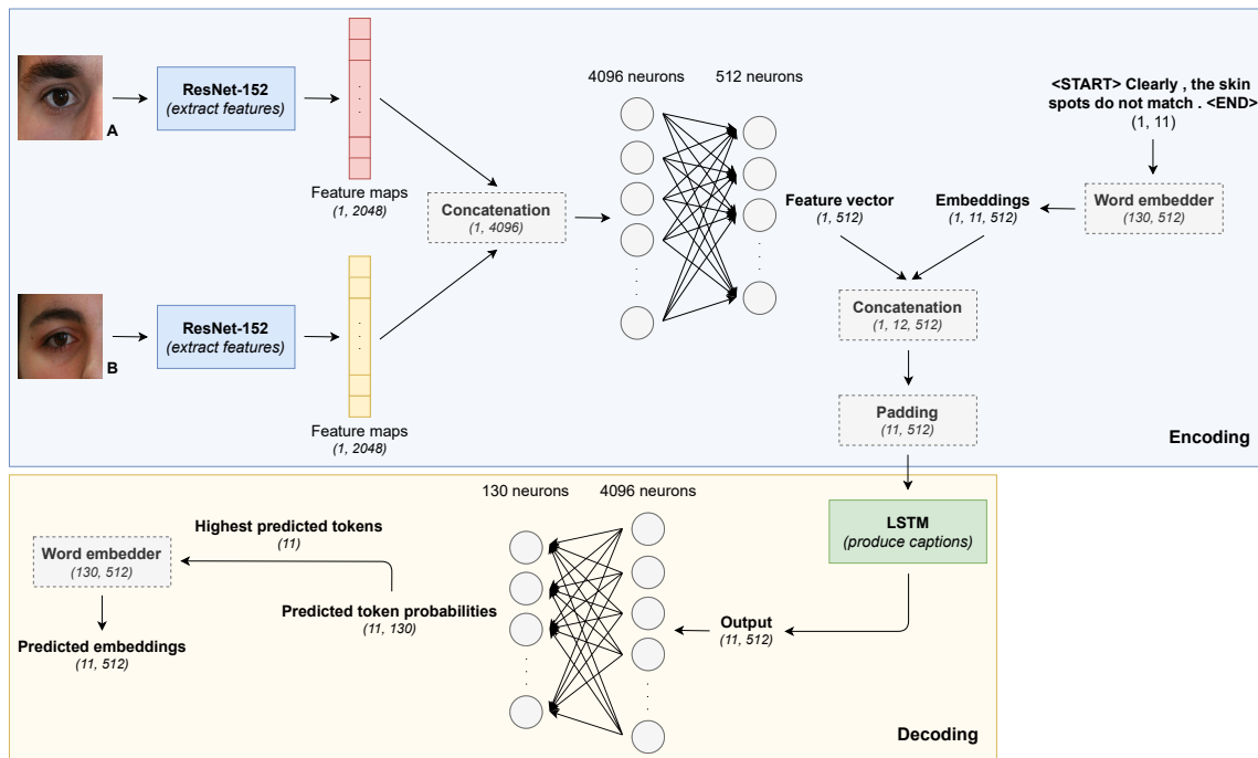
Figure 3.5: Overview of the learning stage of the captioning solution. A given image pair is given to the same CNN, which extracts a feature map for each image. Then, the two feature maps are concatenated lengthwise and given to a couple of linear layers, culminating in a 512-dimensional feature vector. At the same time, the ground-truth caption is embedded and concatenated with the feature vector, leading the resulting tensor through a padding operation (to ensure consistency). Next, the LSTM receives the padded tensor and tries to output the most likely tokens (that make up a caption). Finally, the predicted tokens are encoded so as to retrieve the corresponding embedding, which can naturally be compared to the ground-truth embedding for learning purposes.
