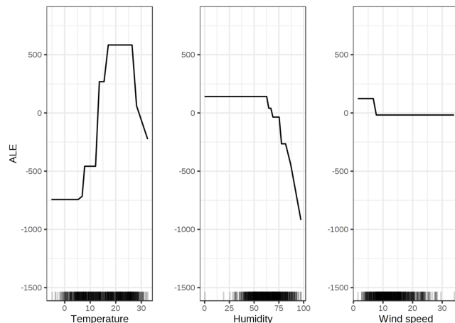
Figure 2.17: Three ALE plots from a regression model with three independent variables and one, dependent variable [Mol19]. As per the trained model, the temperature and humidity’s influence outweighs that of the wind speed.
