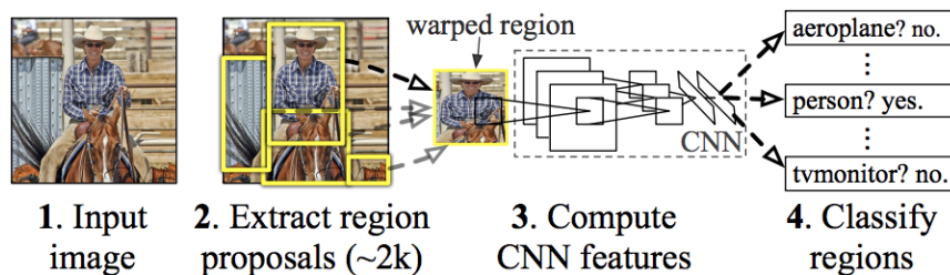
Figure 2.4: R-CNN pipeline [DM14]. The framework uses selective search to create region proposals, which are later fed to a CNN that extracts features. Then, a trained SVM classifies the feature maps as describing a known object or not.
