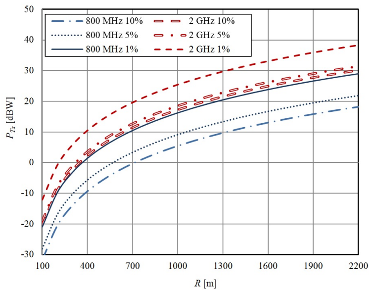
Fig. 6 Normalized P_{Tx} required to achieve a constant average SINR (dB), near the maximum, as a function of the cell radius at 800 MHz and 2 GHz for \alpha = 1 .
