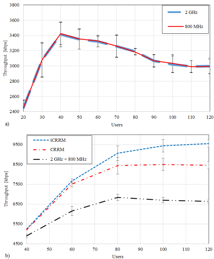
Fig. 7 Average throughput vs. number of users for different cell radii, a) in the absence and b) presence of CRRM and iCRRM at 800 MHz and 2 GHz, with R = 1000 m.
