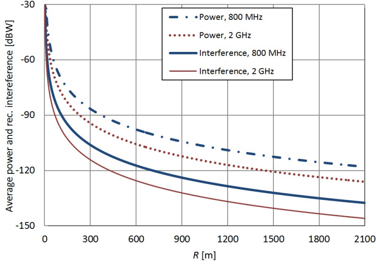
Fig. 4 Average power and interference (dBW) within a cell as a function of the inter-cell distance (m) with P_{Tx} = 1 dBW and \alpha = 1
