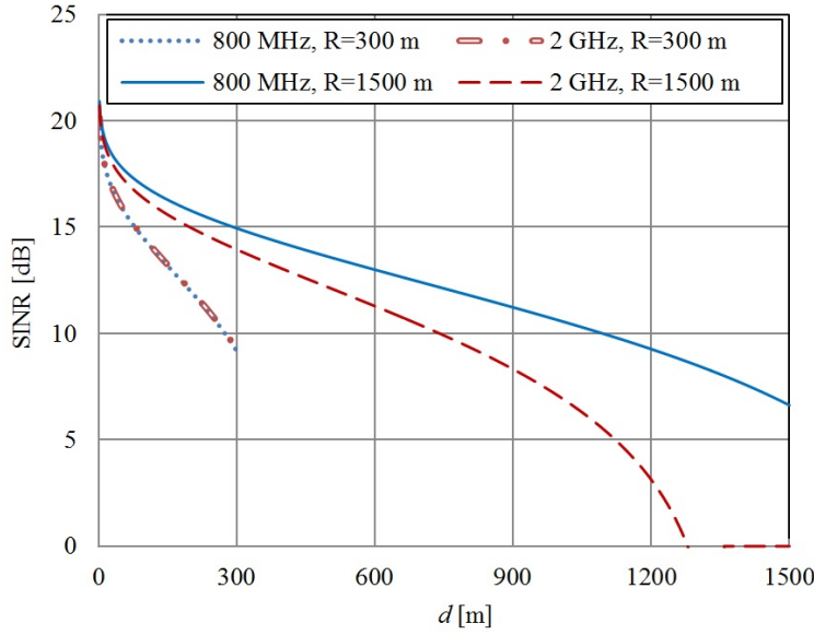
Fig. 3 SINR as a function of the UE-BS distance for two cell radii ( R \in \{300, 1500\} m ) and P_{Tx} = 1 dBW.
