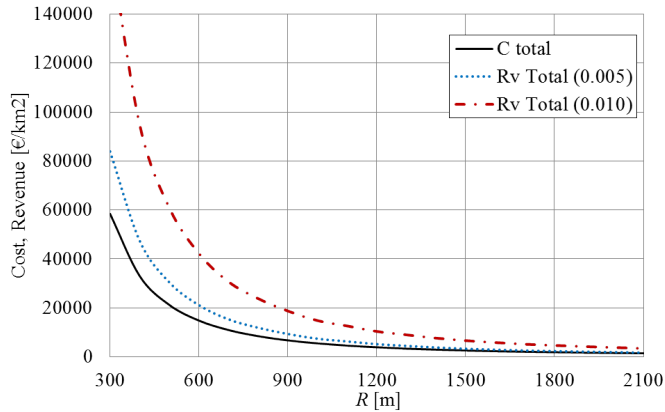
Fig. 9 Total cost and revenue versus R with different R_{R_b}[\text{€/min}] .
