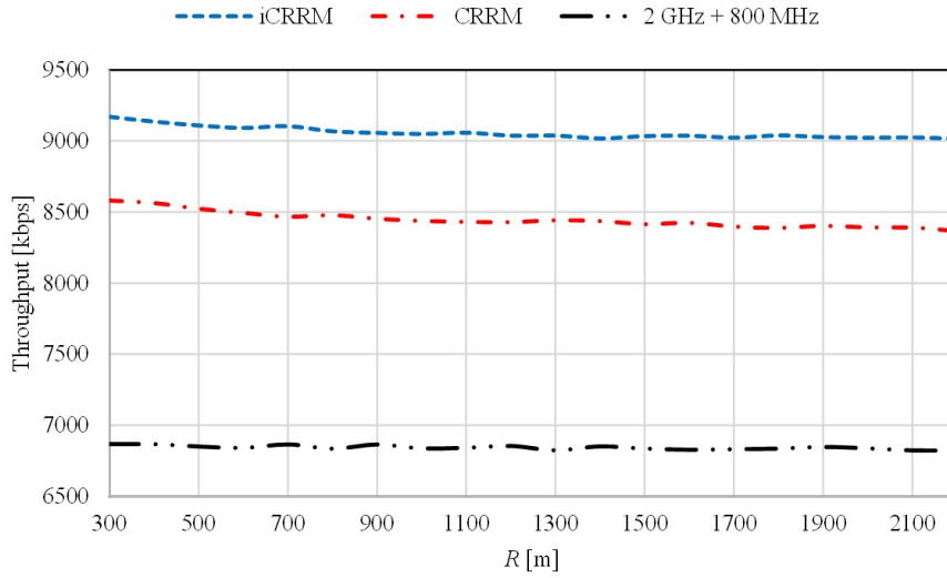
Fig. 8 Comparison of the average throughput as a function of cell radius, R , for 80 users.
