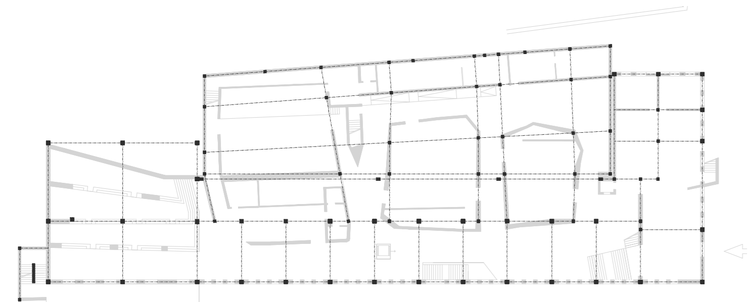
STRUCTURE SCHEME
