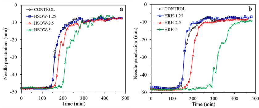
Fig. 3. Setting time for percentage replacement of cement by hydrochars from stabilized organic waste (a) and from rice husk (b).
