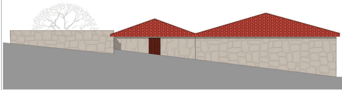
SOUTH FACADE 1:200
