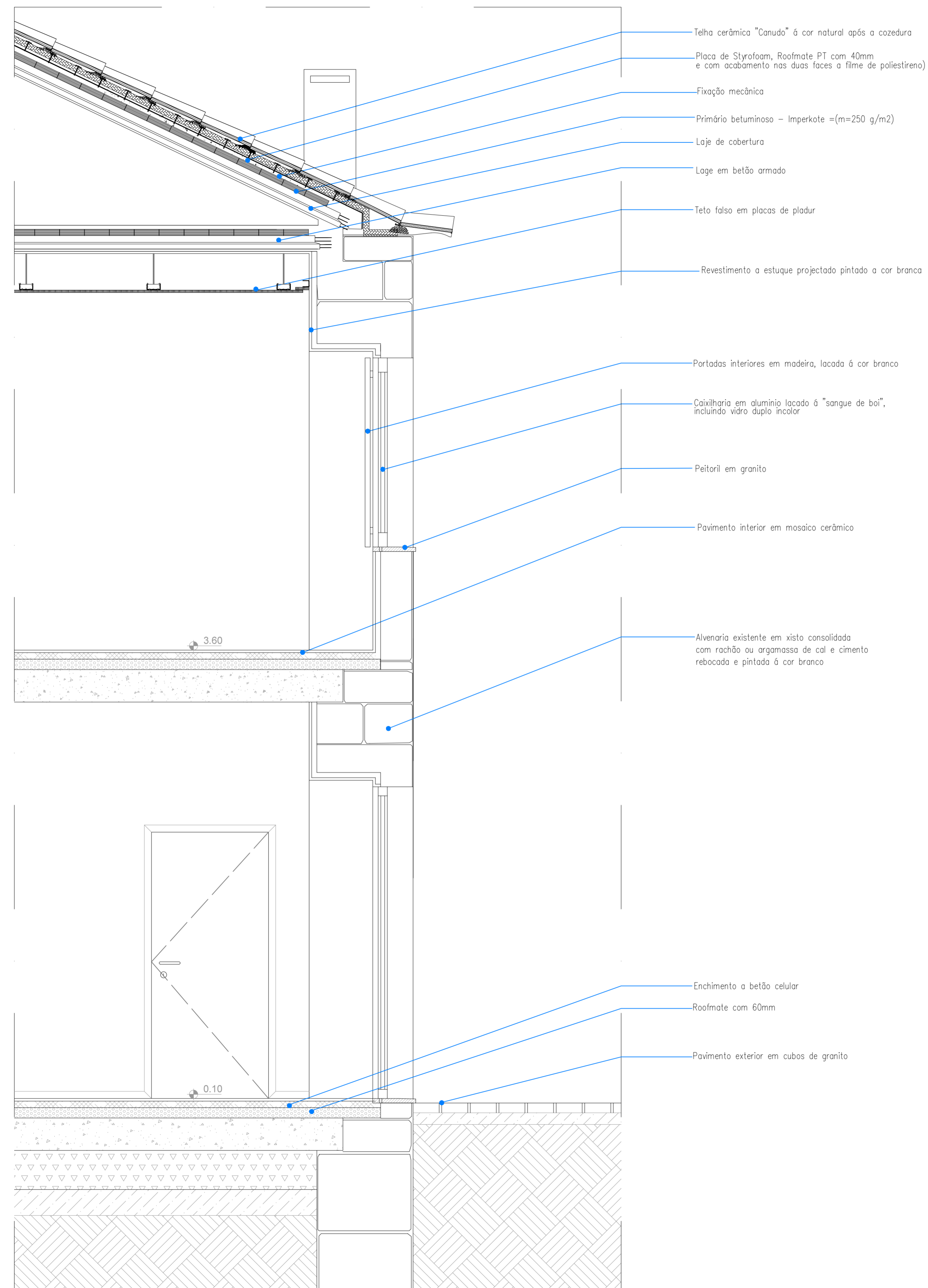
PORMENOR 1 Esc:1/20
