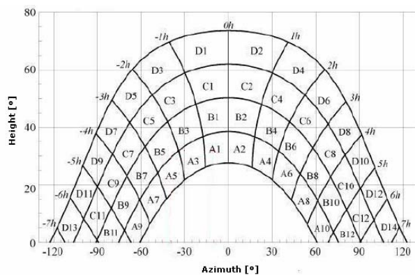
Fig. 4 Division by zones of the sun position, according to the month, day and time (latitude 40° North).
