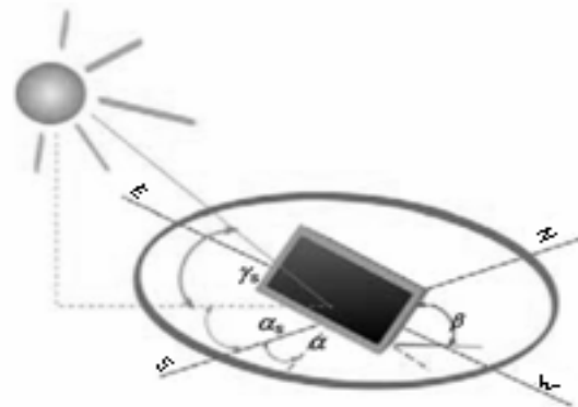
Fig. 1 Description of angles for solar technology.
