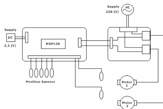
Fig. 6 Electrical scheme of the control system.
