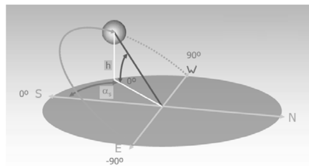
Fig. 2 Sun path.
