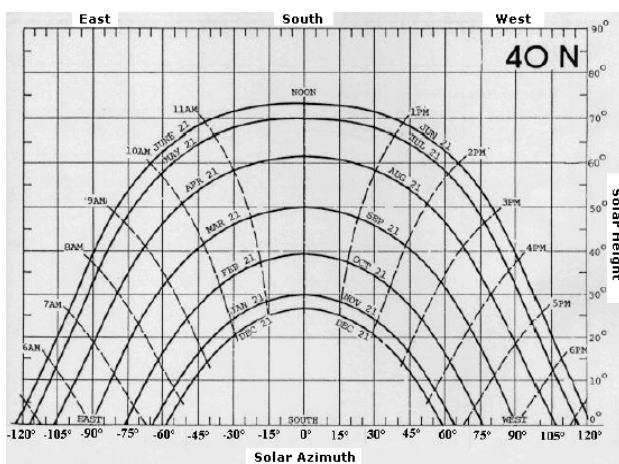
Fig. 3 Sun apparent position, according to the month, day and time for latitude 40° North.
