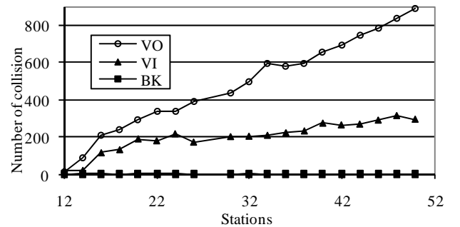
Figure 6. Number of collision with mixtures of applications.
