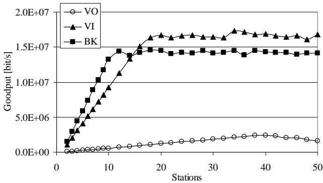
Figure 4. Goodput as a function of the number of node for VO, VI, and BK applications.
