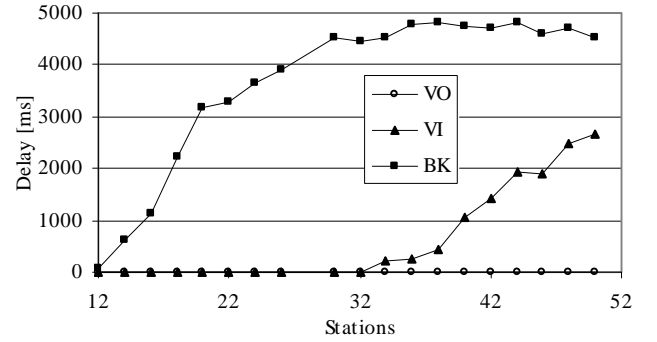
Figure 5. Delay with mixtures of applications.
