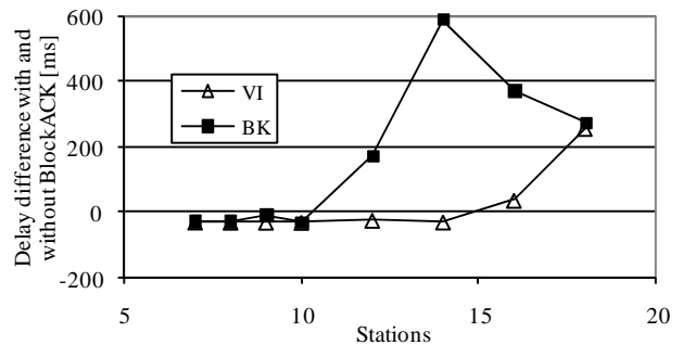
Figure 14. Difference for delay with and without Block ACK.
