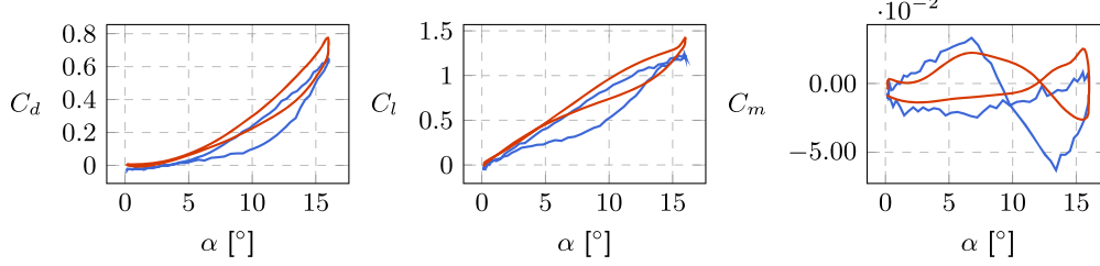
Fig. 9. Case 196 from the test pool with R^2 = 0.9392 .
