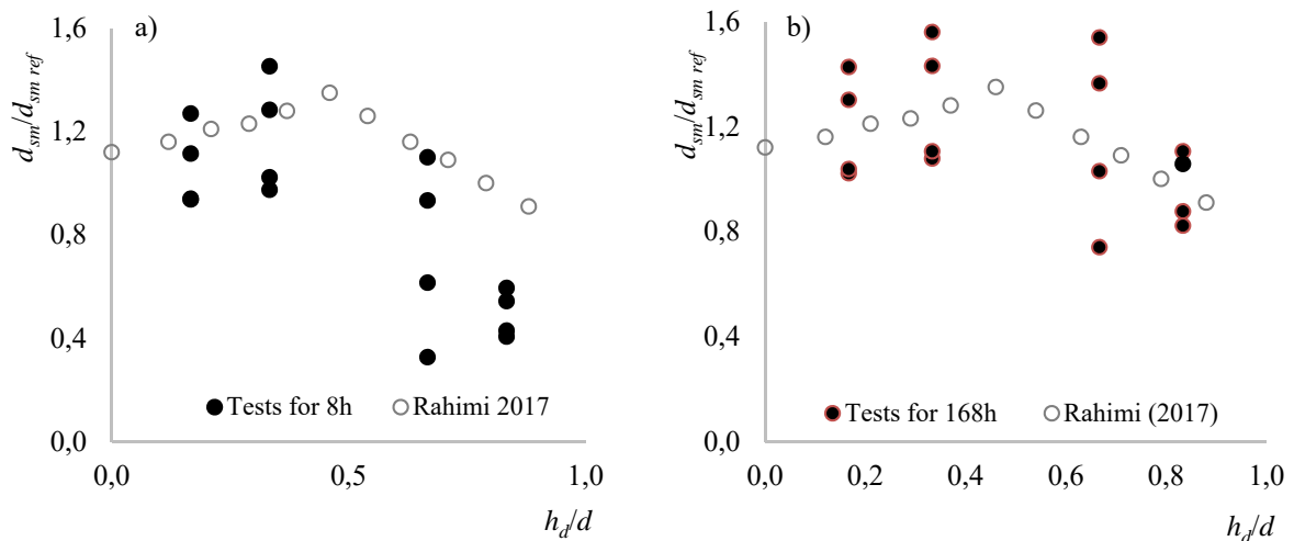
Figure 6. Variation of d_{sm}/d_{ref} vs. h_d/d : a) for t_d=8h ; b) for t_d=168h
