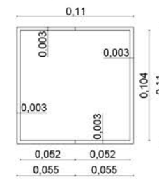
VISTA FRONTAL
