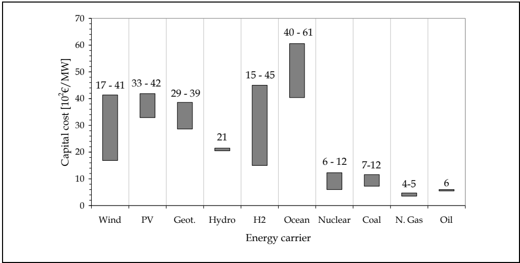
Fig. 5. Values range of capital cost ( 10^2\text{€/MW} ) for each energy carrier.
