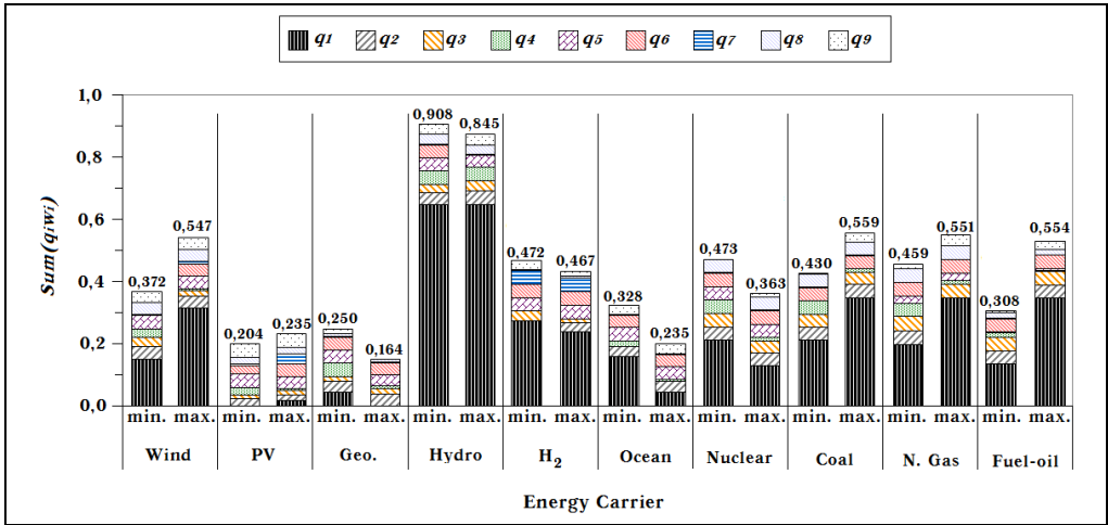
Fig. 12. Maximum and minimum values range of sustainability index for each energy carrier system - Case Scenario 2 (Highest weighting factor for efficiency indicator: q_1 ).
