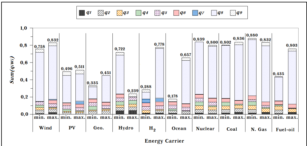
Fig. 16. Maximum and minimum values range of sustainability index for each energy carrier system - Case Scenario 6 (Highest weighting factor for energy payback time indicator: q_8 ).
