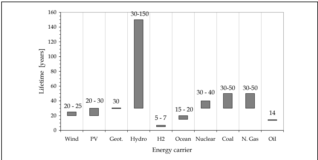
Fig. 3. Values range of lifetime (years) for each energy carrier.
