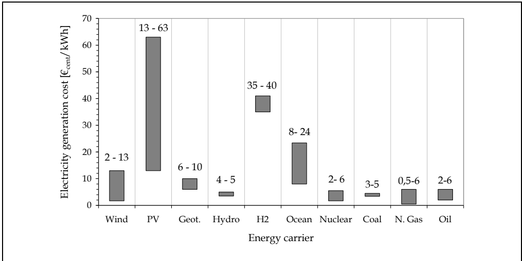
Fig. 6. Values range of electricity generation cost ( \text{€}_{\text{cent}}/\text{kWh} ) for each energy carrier.
