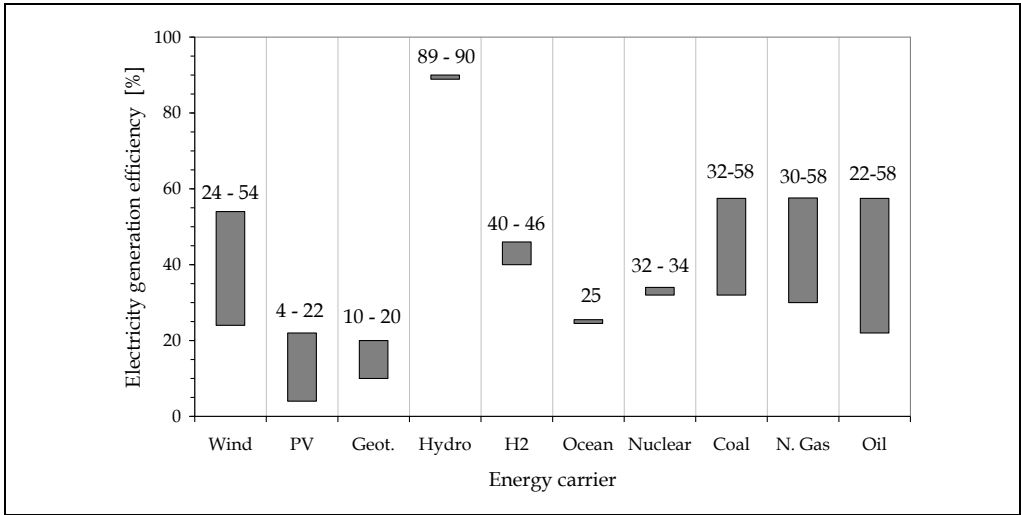
Fig. 2. Values range of electricity generation efficiency (%) for each energy carrier.
