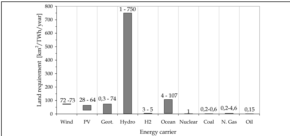
Fig. 8. Values range of land requirements ( \text{km}^2/\text{TWh}/\text{year} ) for each energy carrier.
