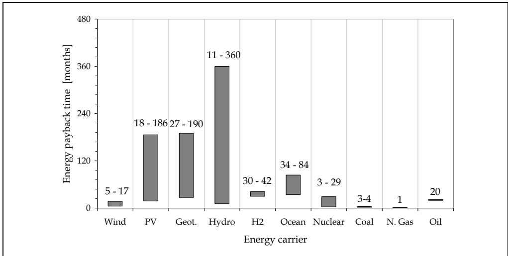
Fig. 4. Values range of energy payback time (months) for each energy carrier.
