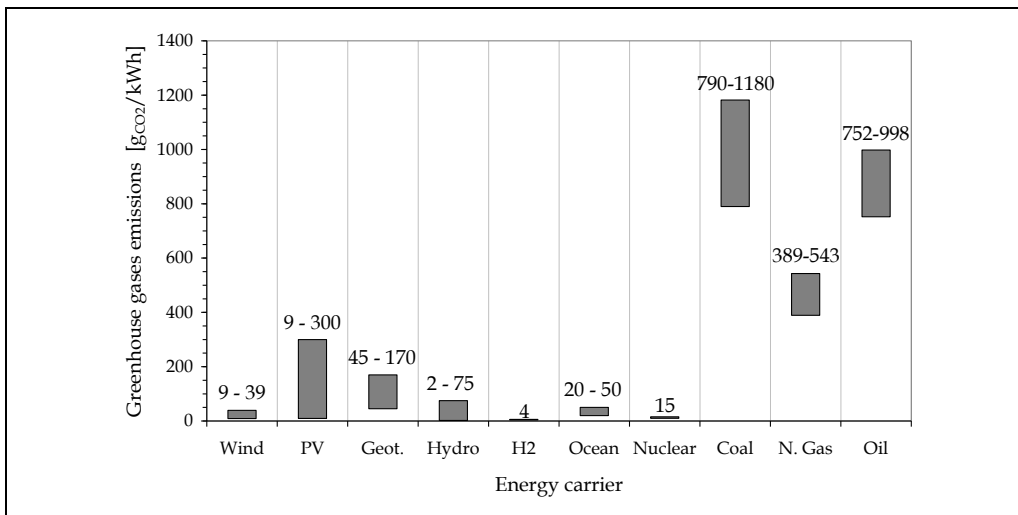
Fig. 7. Values range of greenhouse gases emissions (gCO 2 /kWh) for each energy carrier.
