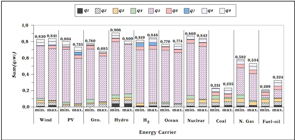
Fig. 15. Maximum and minimum values range of sustainability index for each energy carrier system - Case Scenario 5 (Highest weighting factor for GHG emissions indicator: q_5 ).
