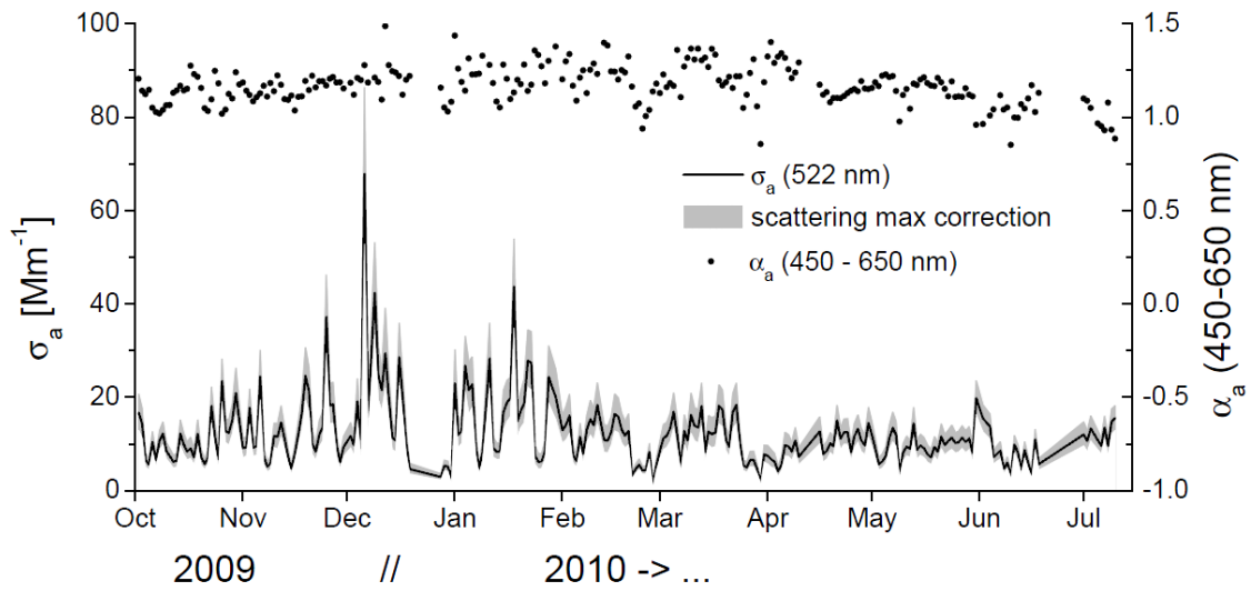
Fig. 2: Time series of the \sigma_a (522 nm) and the \alpha_a (450-650 nm) for all data set (24 h averages).
