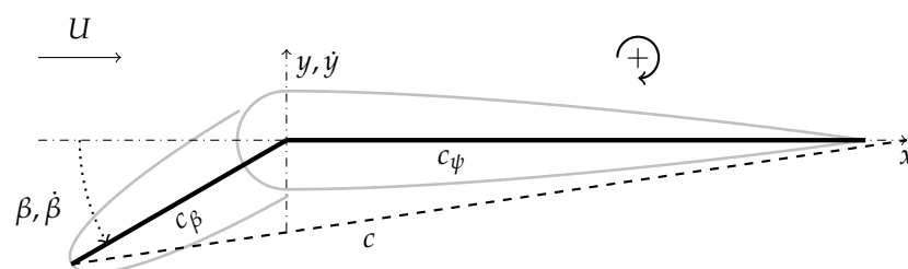
Figure 2. Scheme of NACA0012-IK30 airfoil.
