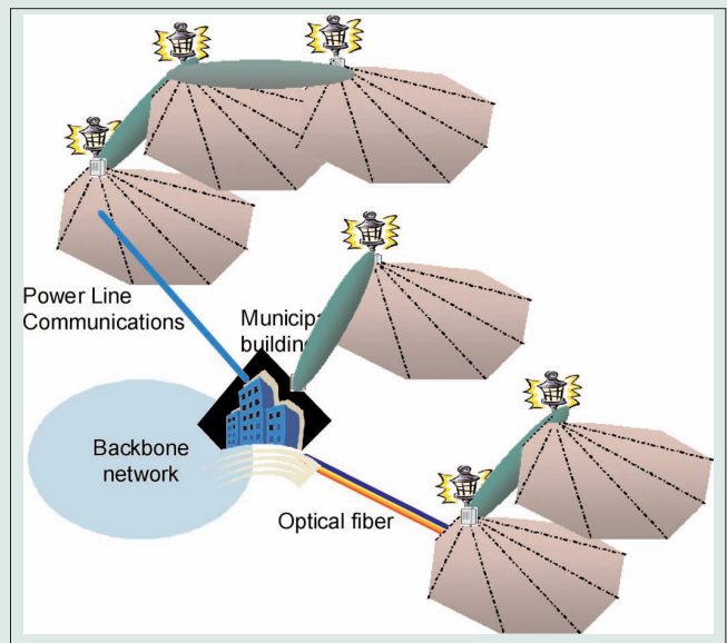
■ Figure 1. Example of interconnection of wireless access points to the backbone network: a municipal building terminates connections based on optical fibers, power line communications, and wireless mesh. Connections can be shared among access points through wireless meshing.
