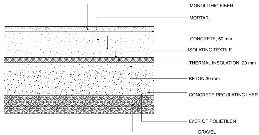
INTERIOR FLOOR DETAIL, PLAN 0
